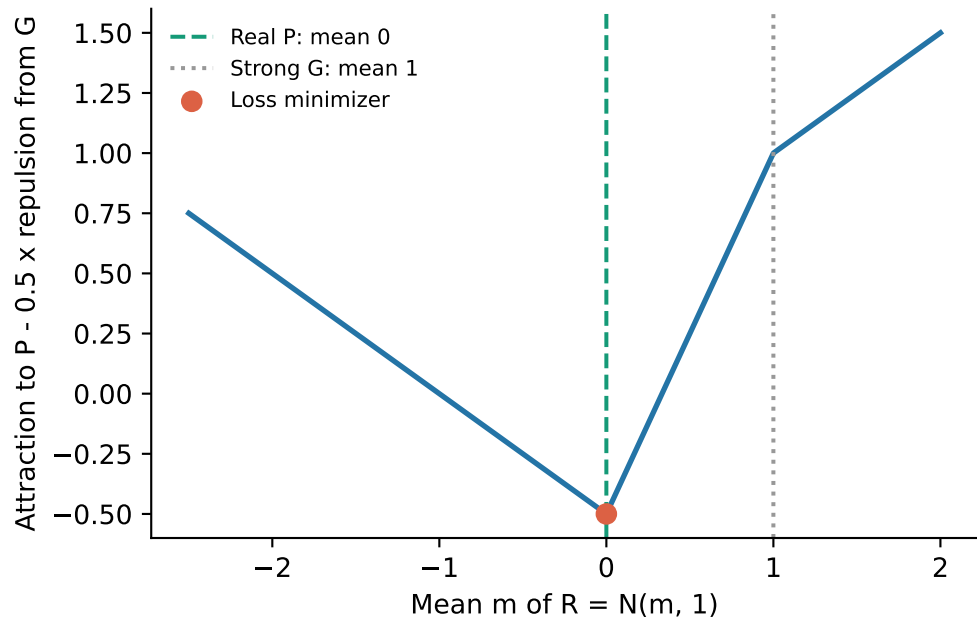
W2 metric: minimum remains at P
