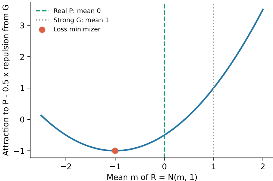
Squared W2: overshoots to mean -1
