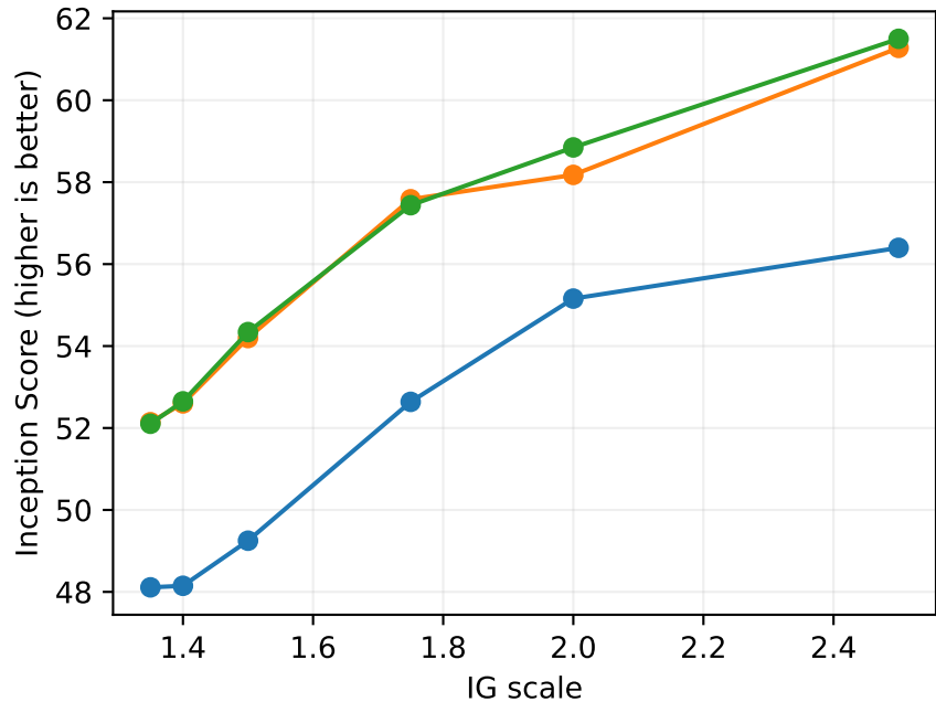
Official SiT-XL/2 + joint IG: eighteen paired discovery points
