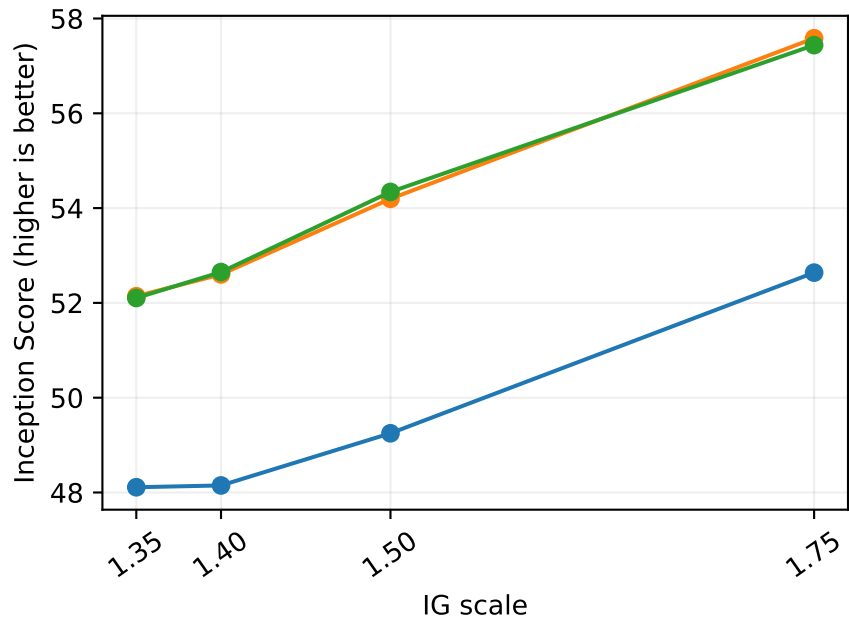
Official SiT-XL/2 + joint IG: paired 1K discovery bank
