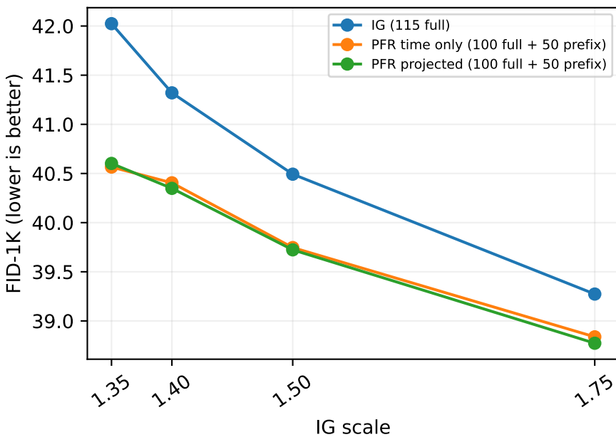
Official SiT-XL/2 + joint IG: paired 1K discovery bank
