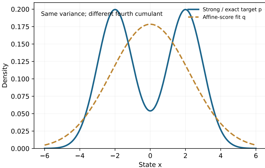
A broad reference need not be Gaussian blur
