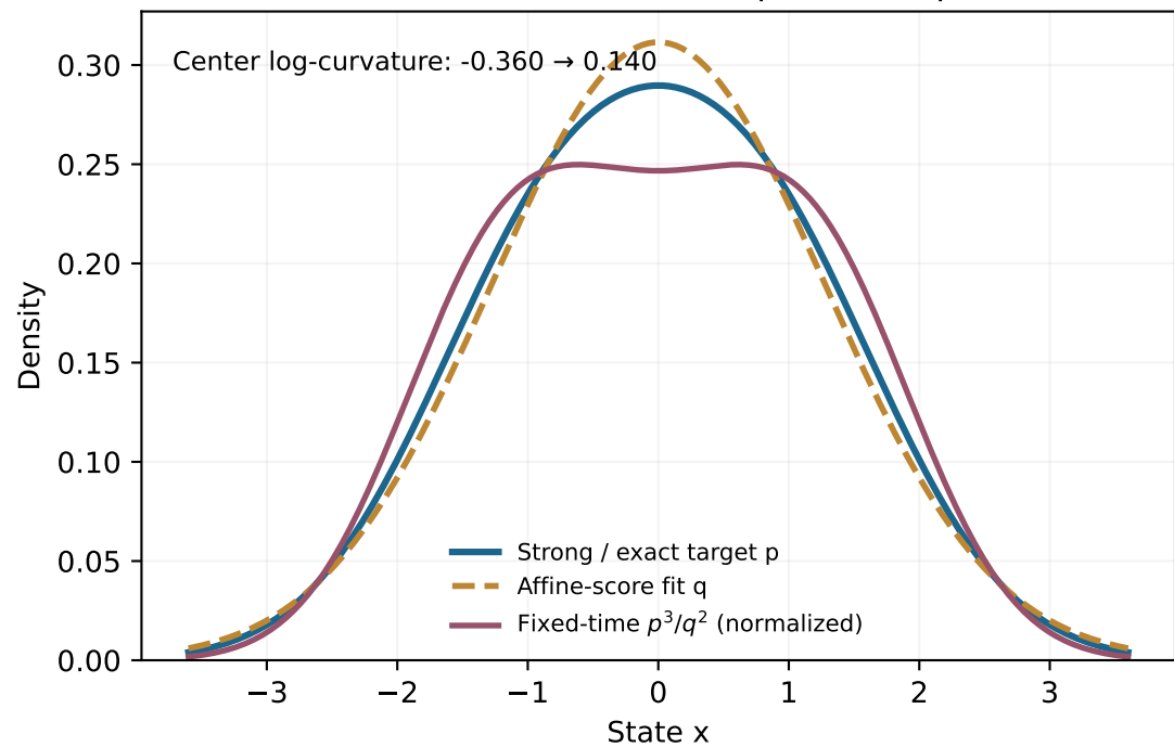
Even an exact unimodal p can be split
