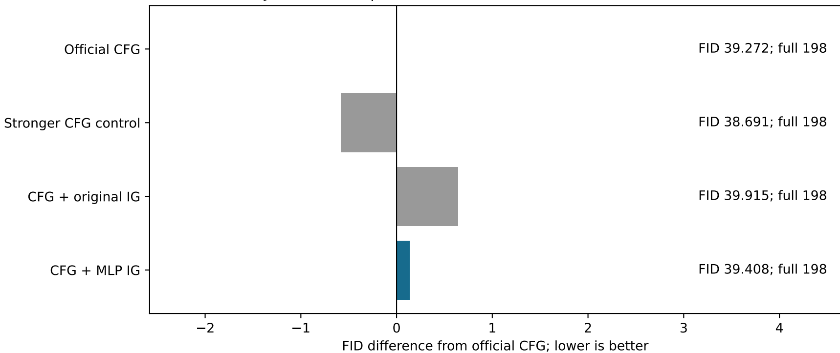
JiT-B/16: new paired 1K, official CFG with retained IG heads
