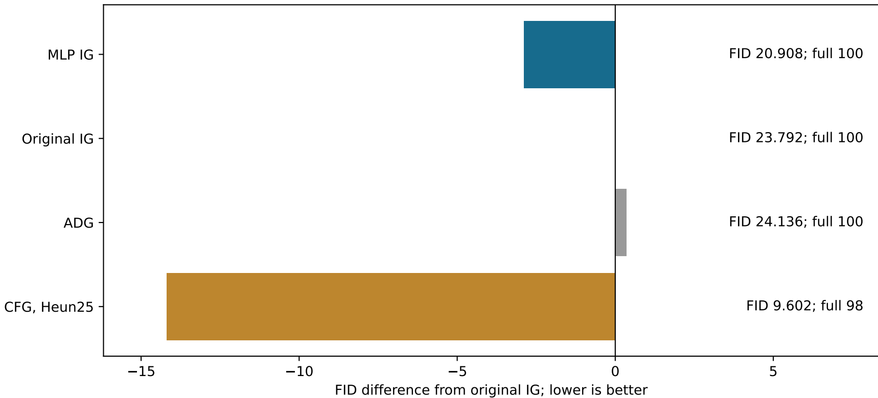
JiT-B/16: independent paired 5K, 98-100 full forwards per image
