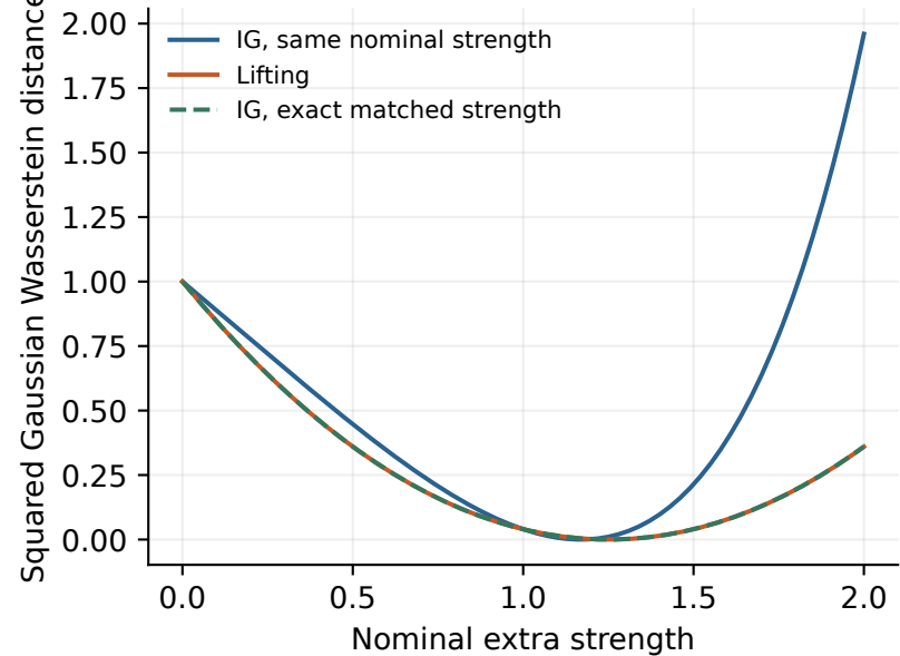
Pointwise gains can be reparameterization
