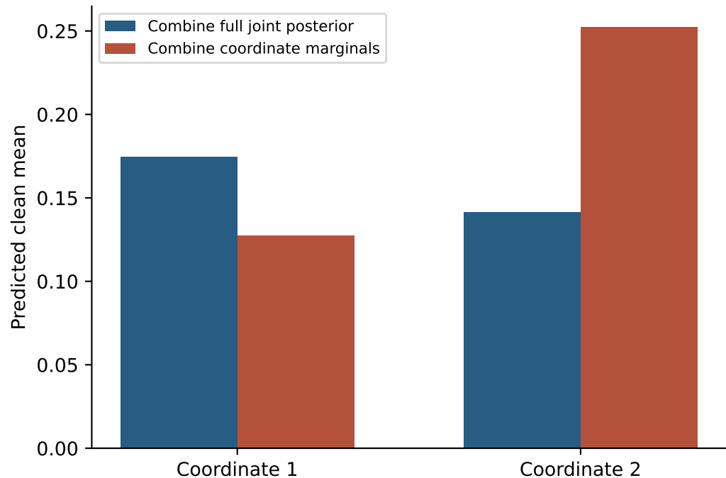
Marginals do not preserve the joint identity
