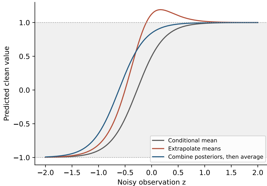
Full clean candidates: \{-1, +1\}
