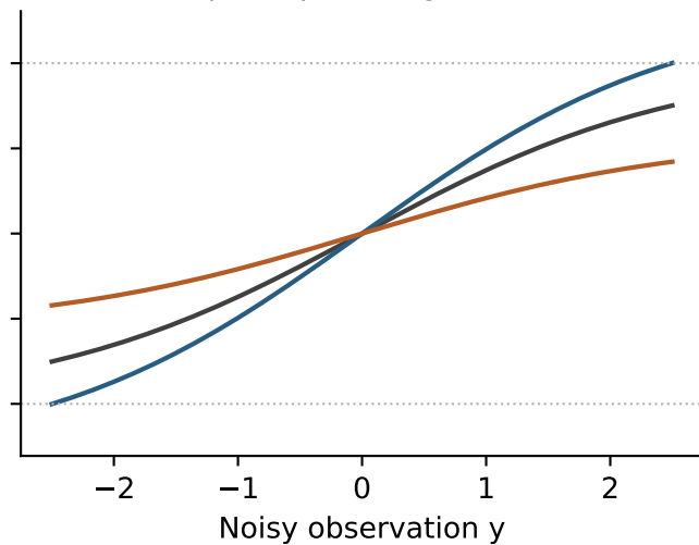
Two-point prior, sigma = 1.6
