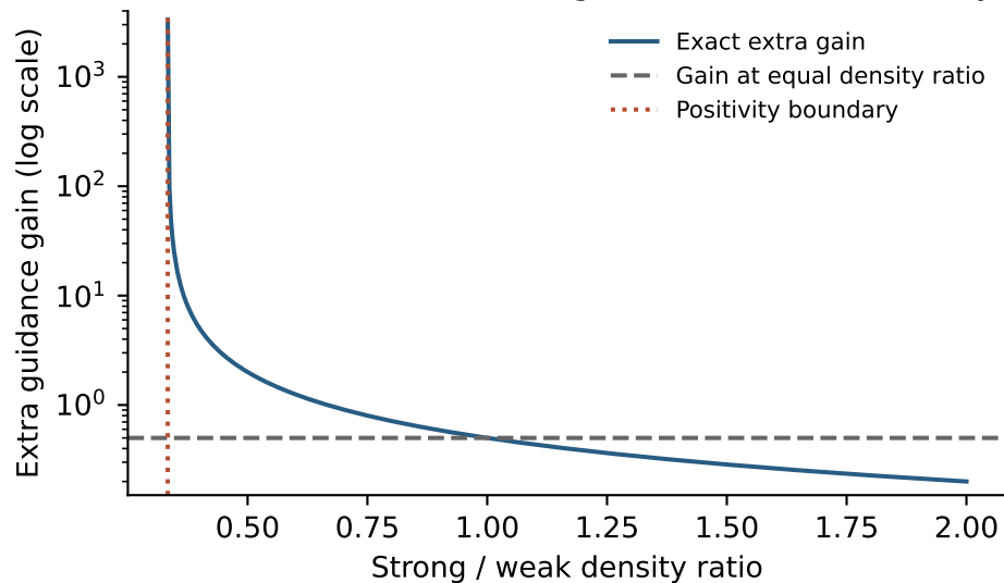
The inverse becomes singular near the boundary
