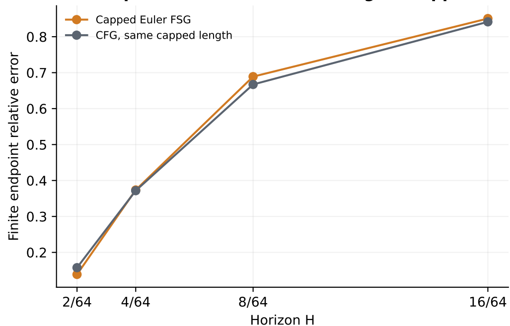
Adapter own Euler-forward target · capped
