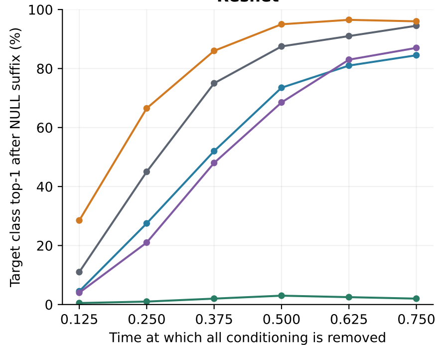
Fixed 200-image bank; every method uses the same noise and labels
