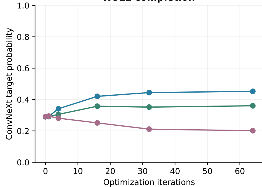
NULL completion
