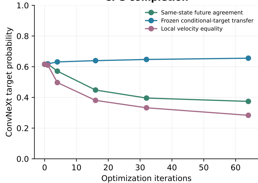
CFG completion
