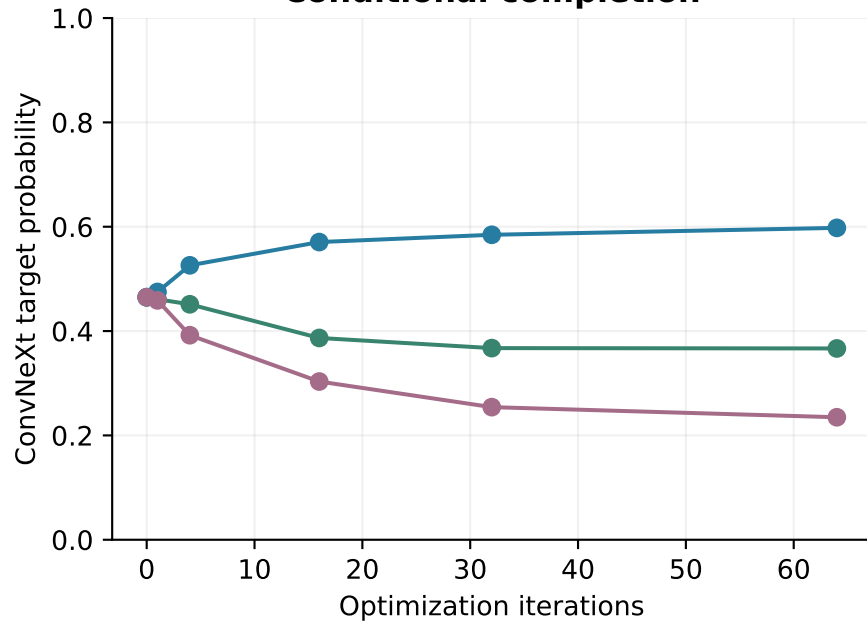
Conditional completion
