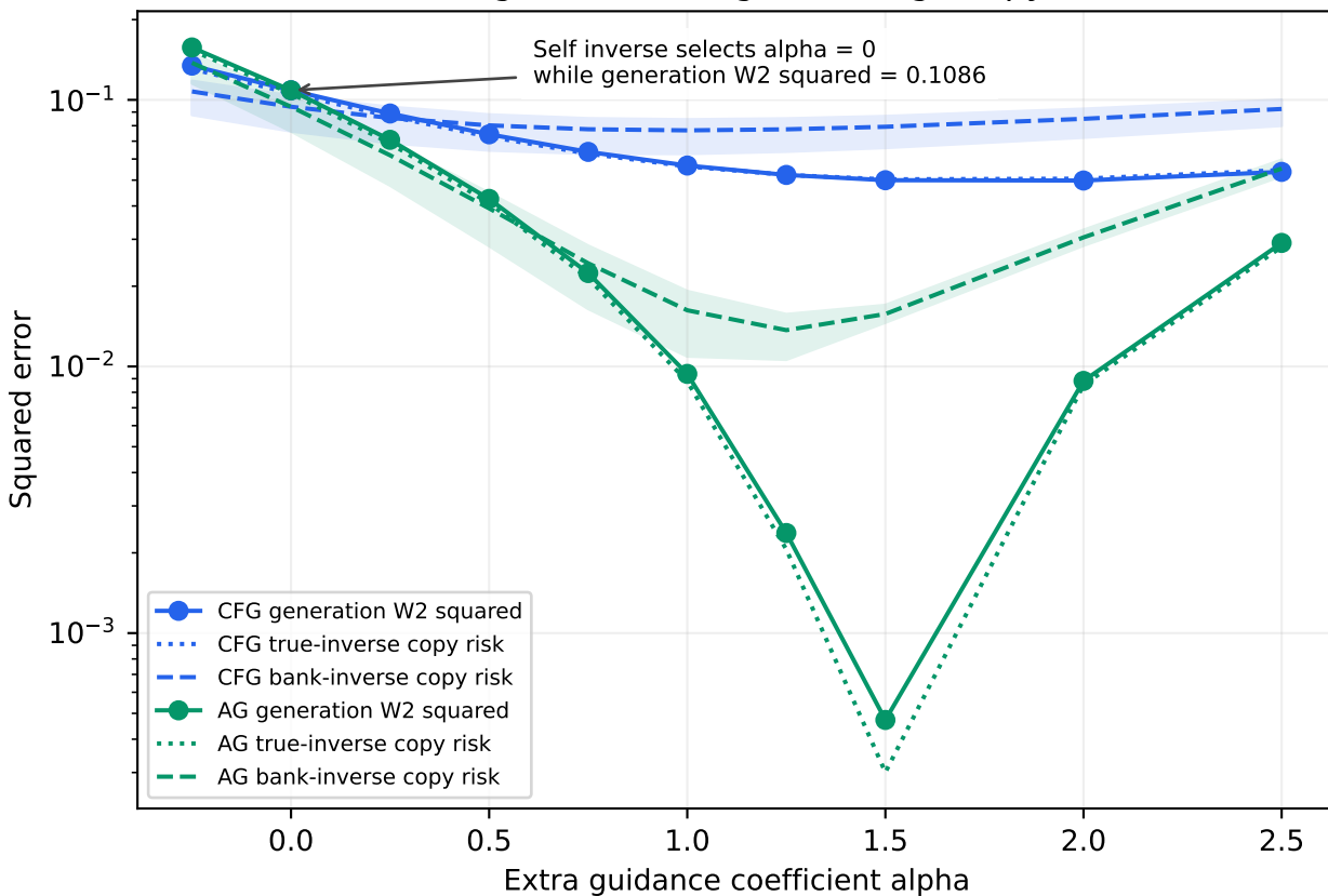
Choose guidance using real-image copy risk
