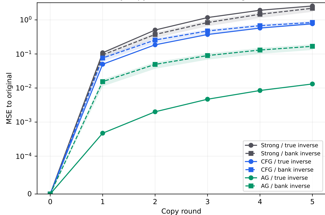
Every copy round: error to the original
