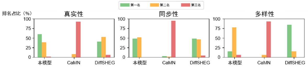
图 5.3 平衡拉丁方设置下的主观排名结果 Figure 5.3 Subjective Ranking Results under Balanced Latin Square Design
