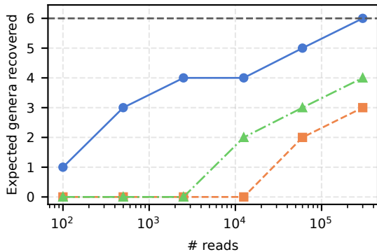
Full-length 18S rRNA protist community (ONT R10.4 sup)
