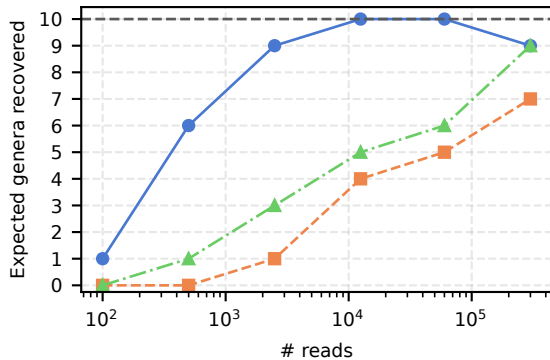
ITS fungal community (ONT R10.4 hac)
