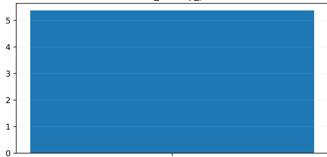
warm_latency_p50
