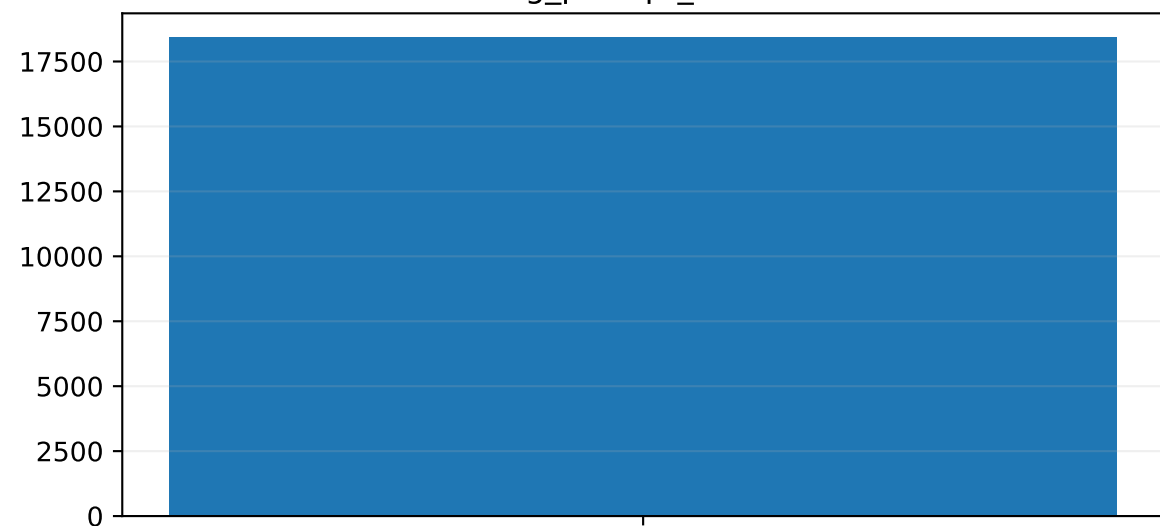
qwen25_coder_7b
