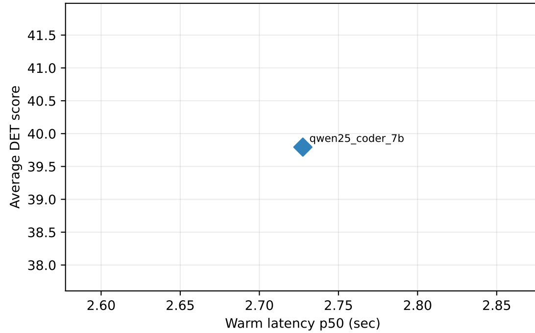
Category 7
