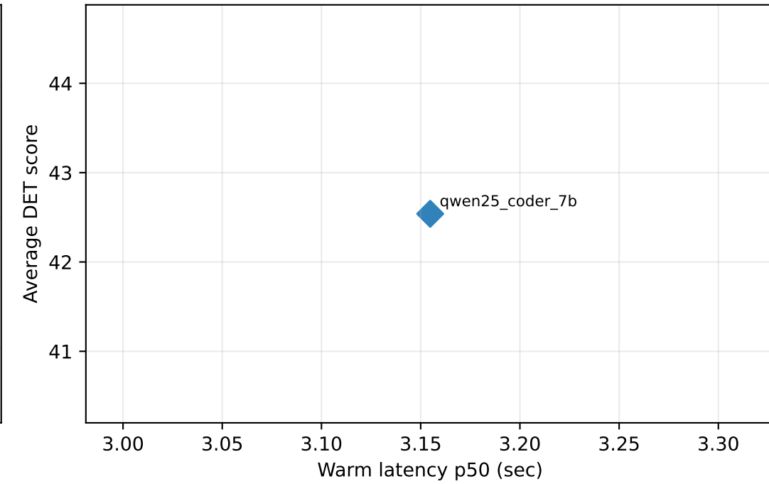
Category 6
