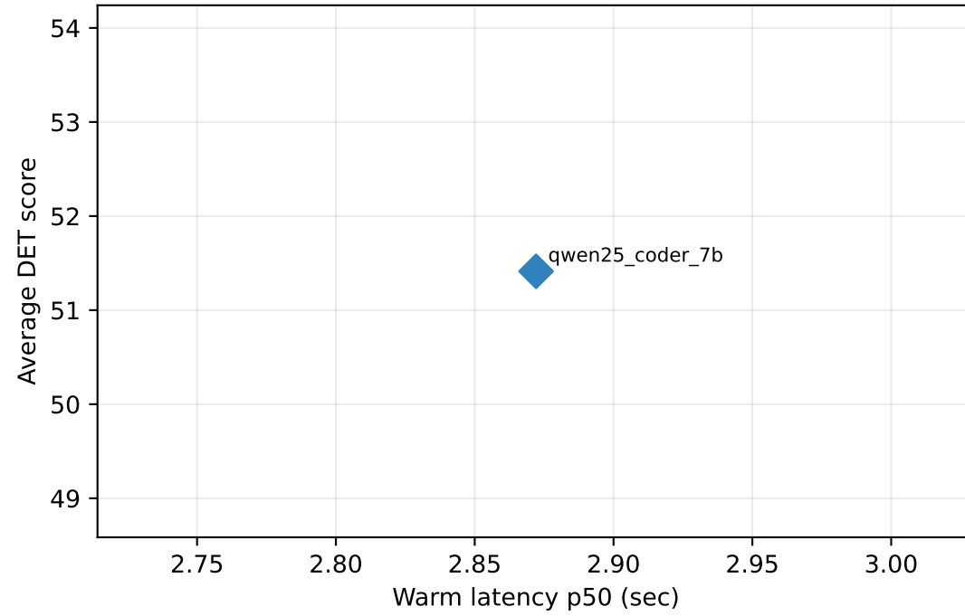
Category 4
