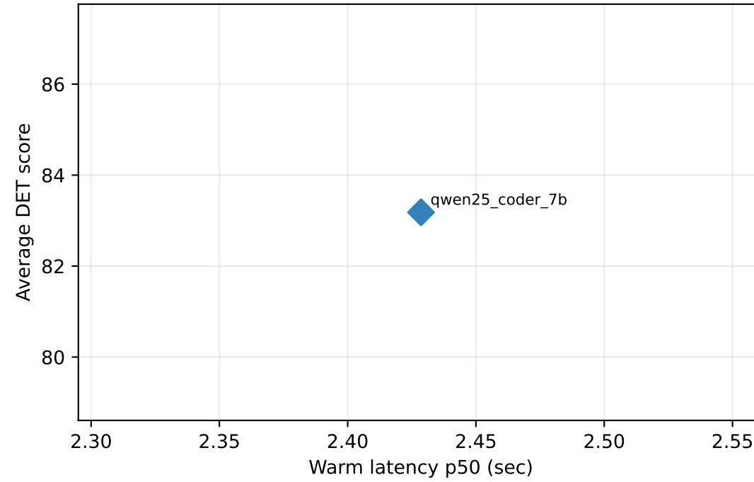
Category 5
