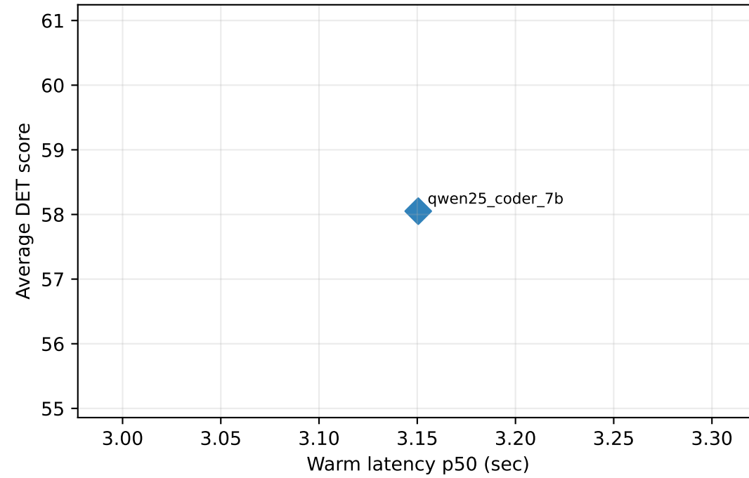
Category 8
