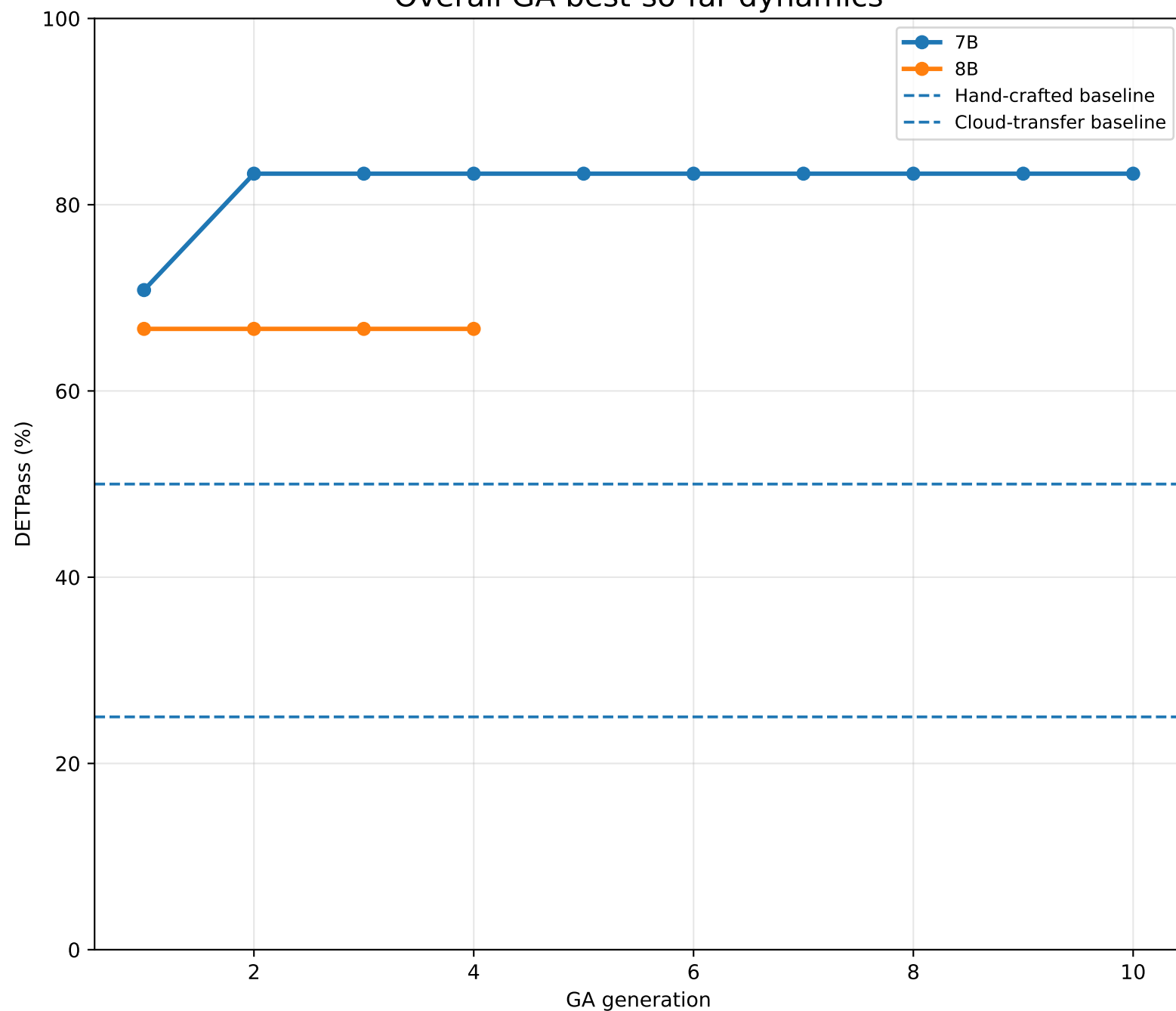
Overall GA best-so-far dynamics
