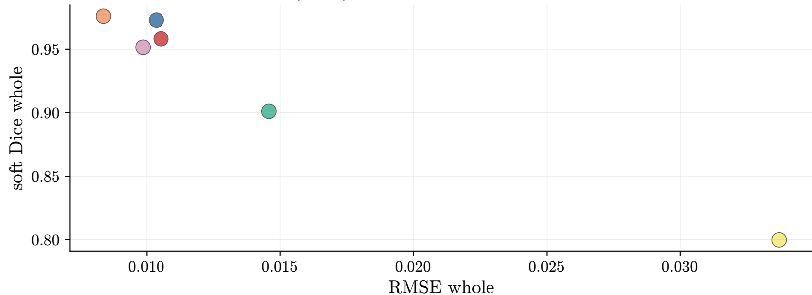
Quality trade-off of selected models
