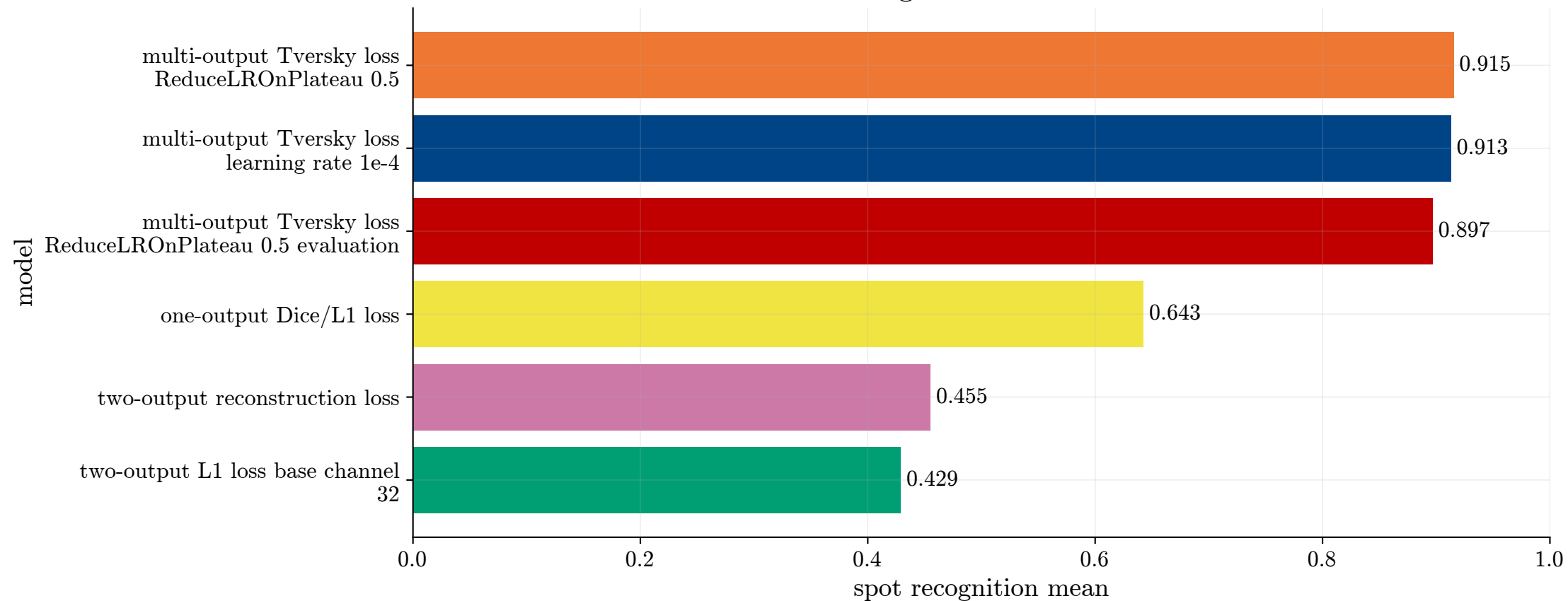
Ranking of different models
