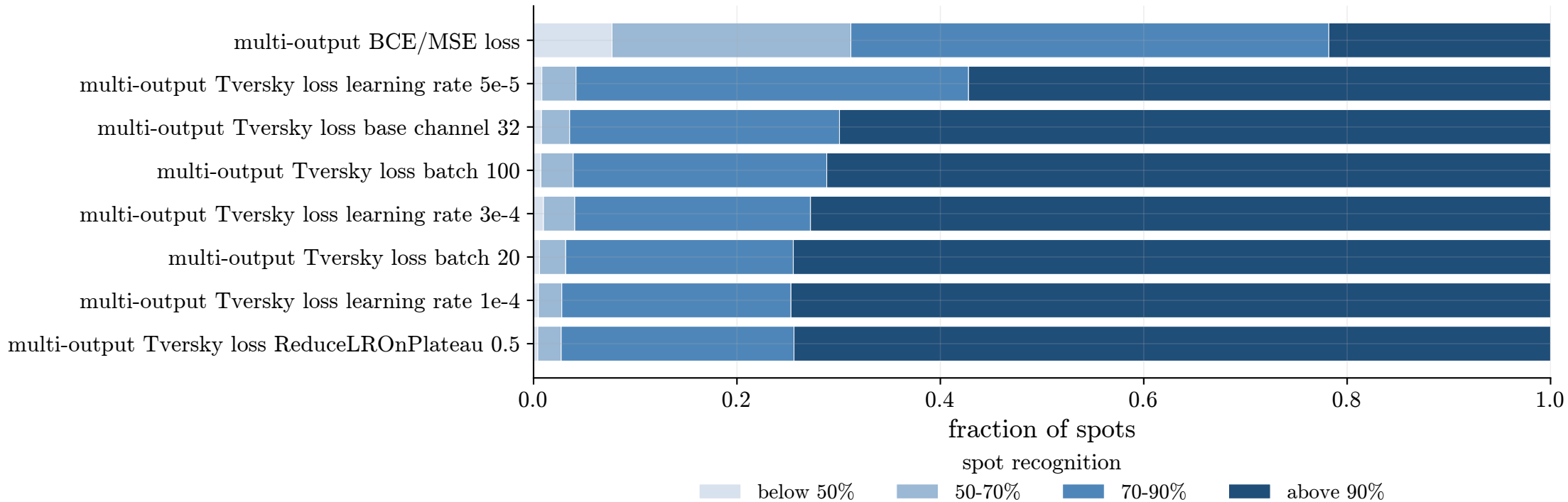
Spot-recognition bin distribution: multi-output
