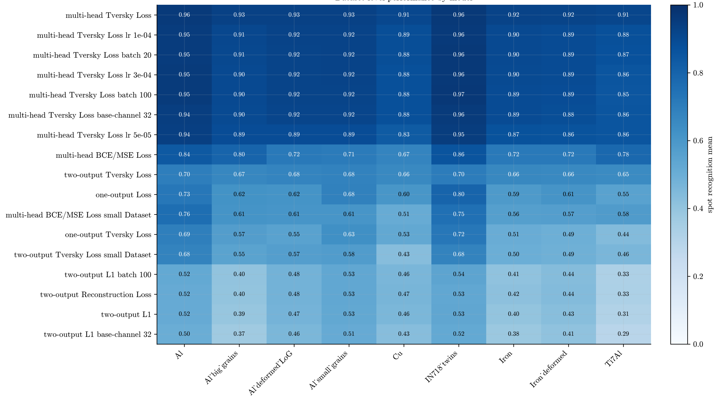
Dataset-level performance by model
