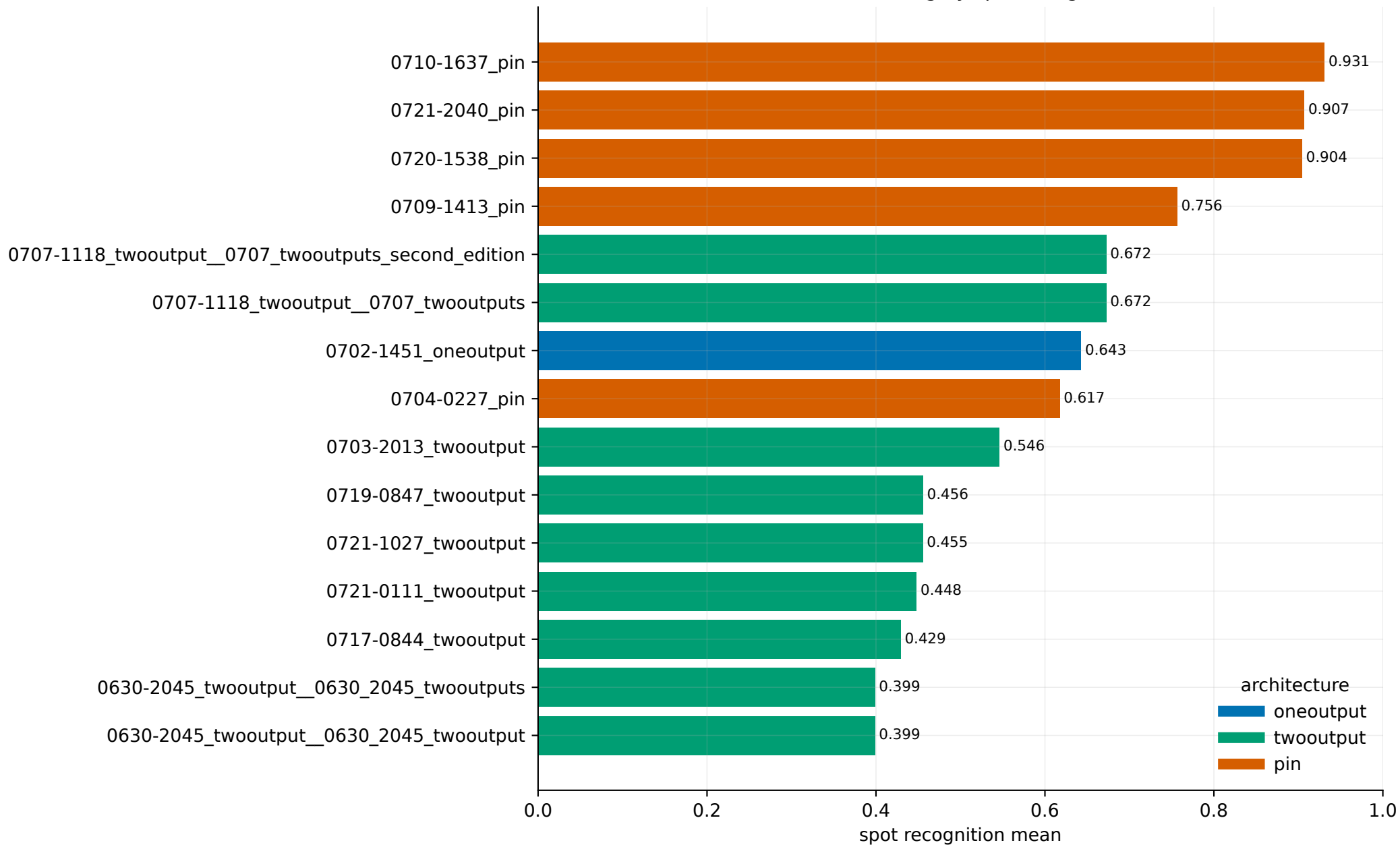
Overall ranking by spot recognition
