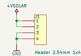
Header 2.54mm 1x4
