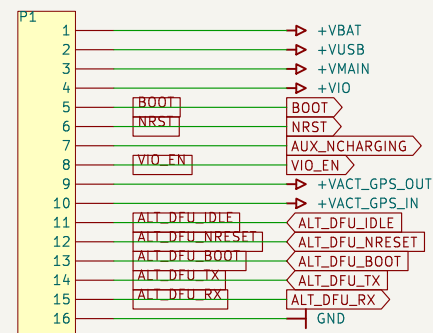
Header 2.54mm 1x16
