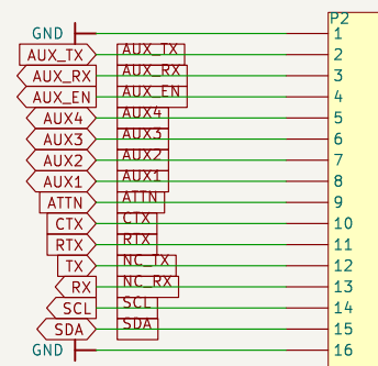
Header 2.54mm 1x16
