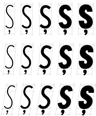
Scommaaccent.ss03
