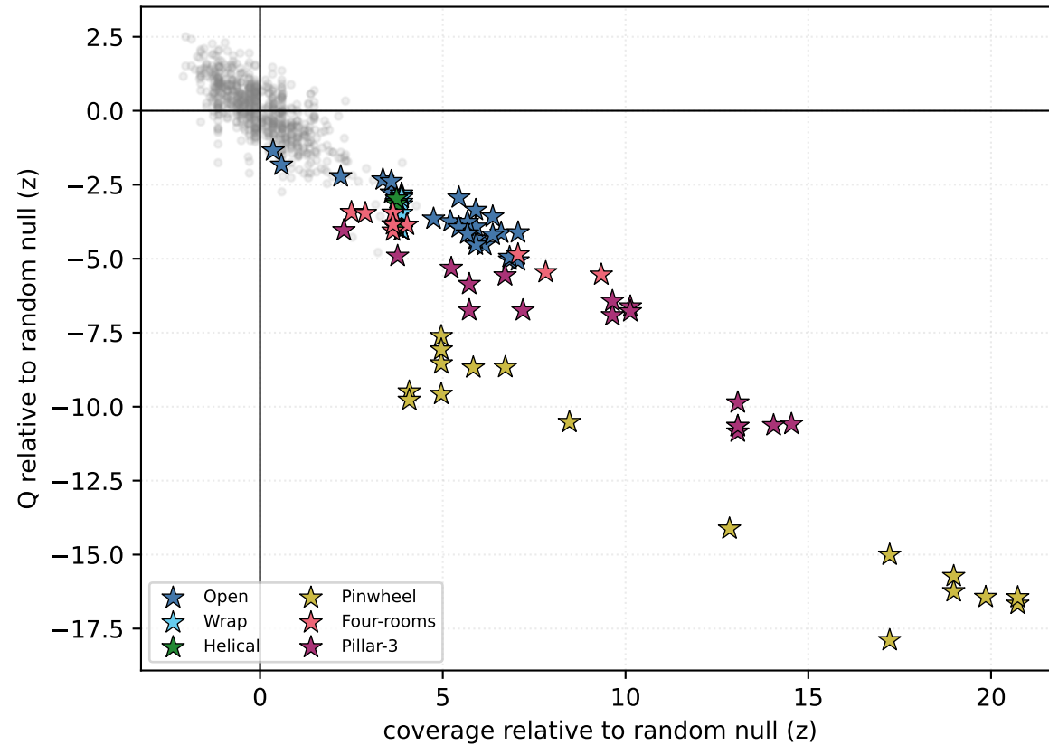
(b) Homing and cross-label specialisation separate
