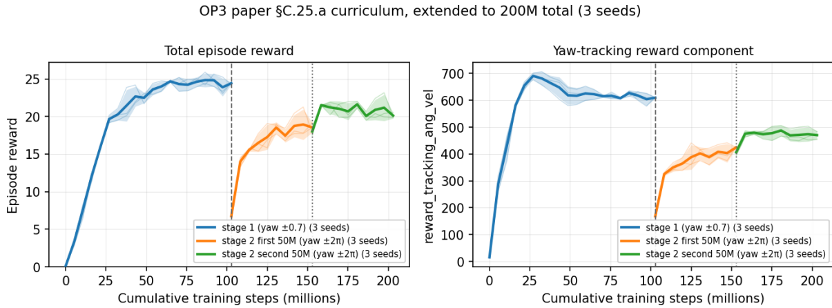
Figure 1: Curriculum reward curves over 200 M cumulative training, 3 seeds (mean \pm \sigma band, thin per-seed lines underneath). Vertical dashed line: stage 1 \rightarrow stage 2a (yaw range \pm 0.7 \rightarrow \pm 2\pi ). Dotted: stage 2a \rightarrow stage 2b. Left: total reward; right: reward_tracking_ang_vel component.
