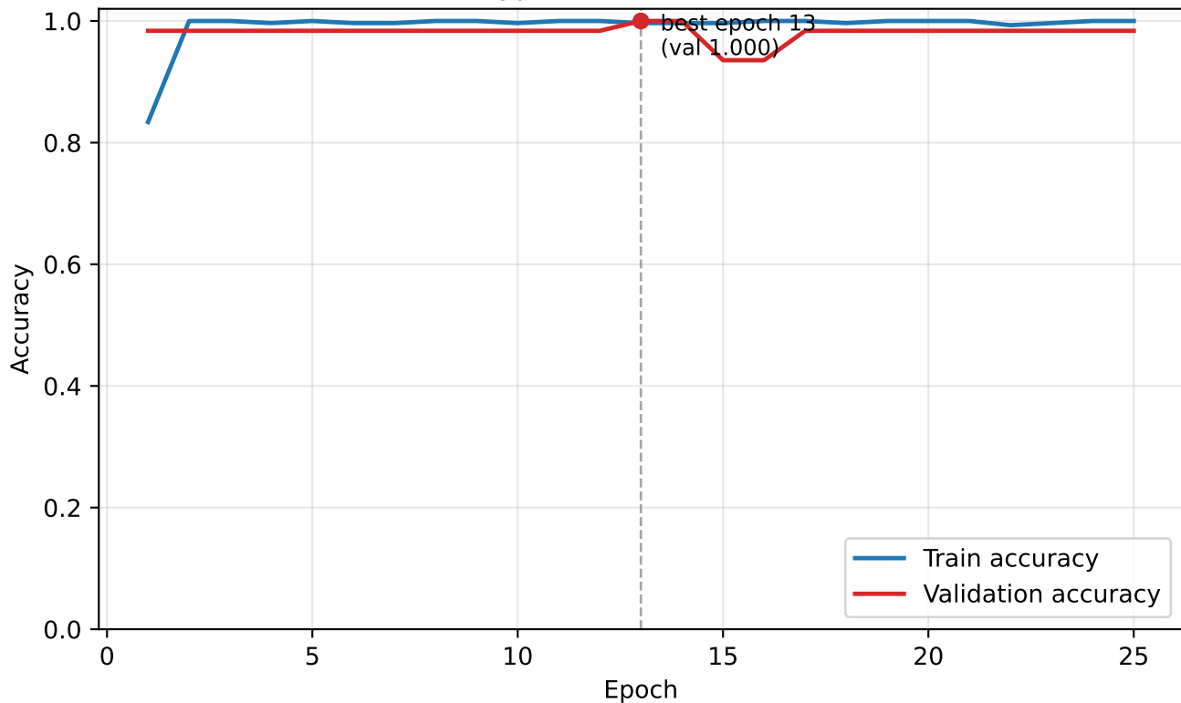
Donation Type Classification (ResNet-18)
