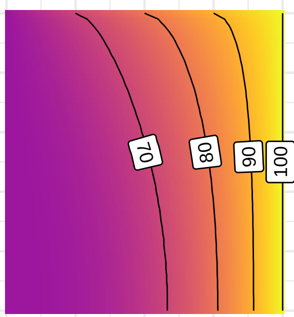
Human AUROC2: 0.8
