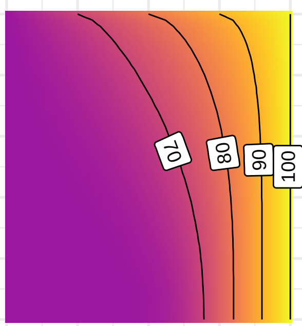
Human Accuracy: 0.6
