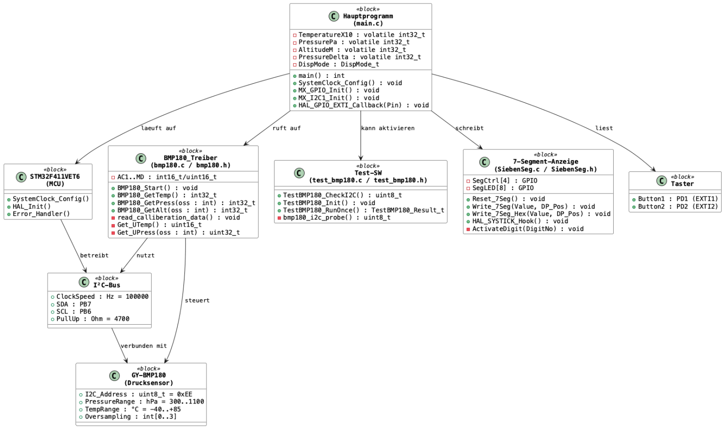
SysML BDD: Luftdruck-Sensor System Block Definition Diagram
