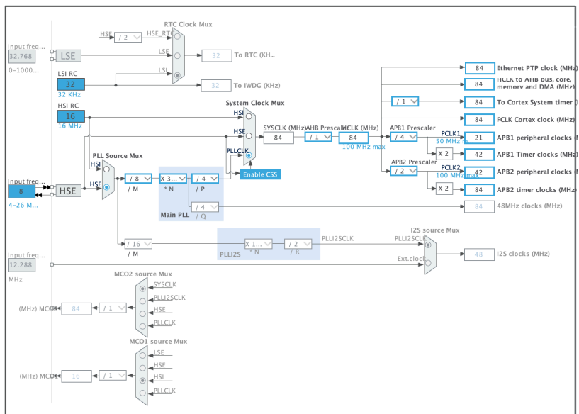
Figure 2: CubeMX Clock Konfiguration
