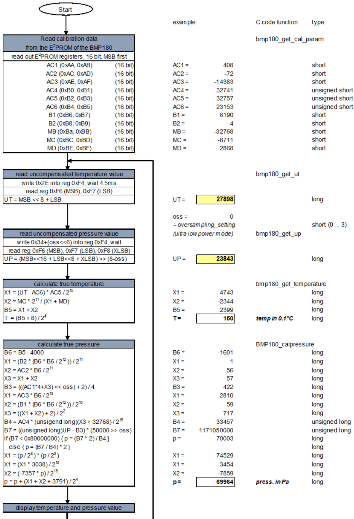
Figure 4: Algorithm for pressure and temperature measurement
