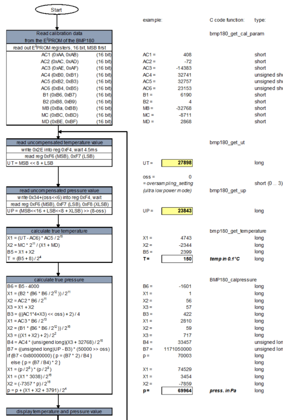
Figure 4: Algorithm for pressure and temperature measurement
