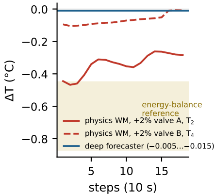
(a) valve-step response
