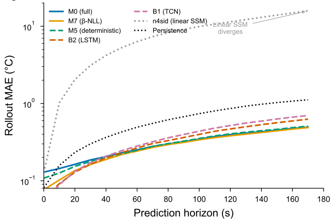
Model comparison: rollout error growth
