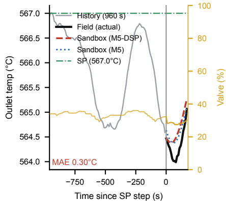
a Large SP step ( |\Delta SP|=3.0^{\circ}\text{C} )
