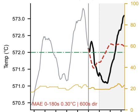
c Calm baseline ( |\Delta SP|=0.0^{\circ}\text{C} )
