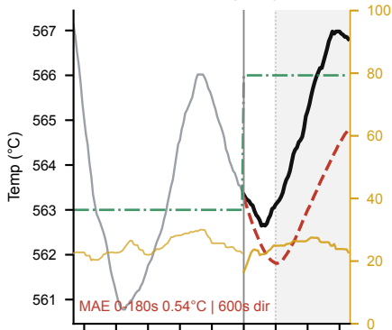
b Medium SP step ( |\Delta SP|=3.0^{\circ}\text{C} )
