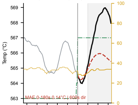
a Large SP step ( |\Delta SP|=3.0^{\circ}\text{C} )
