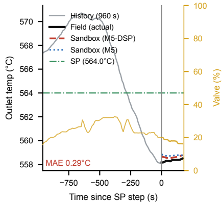
a Large SP step ( |\Delta SP|=3.2^{\circ}\text{C} )
