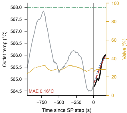
b Medium SP step ( |\Delta SP|=2.1^{\circ}\text{C} )
