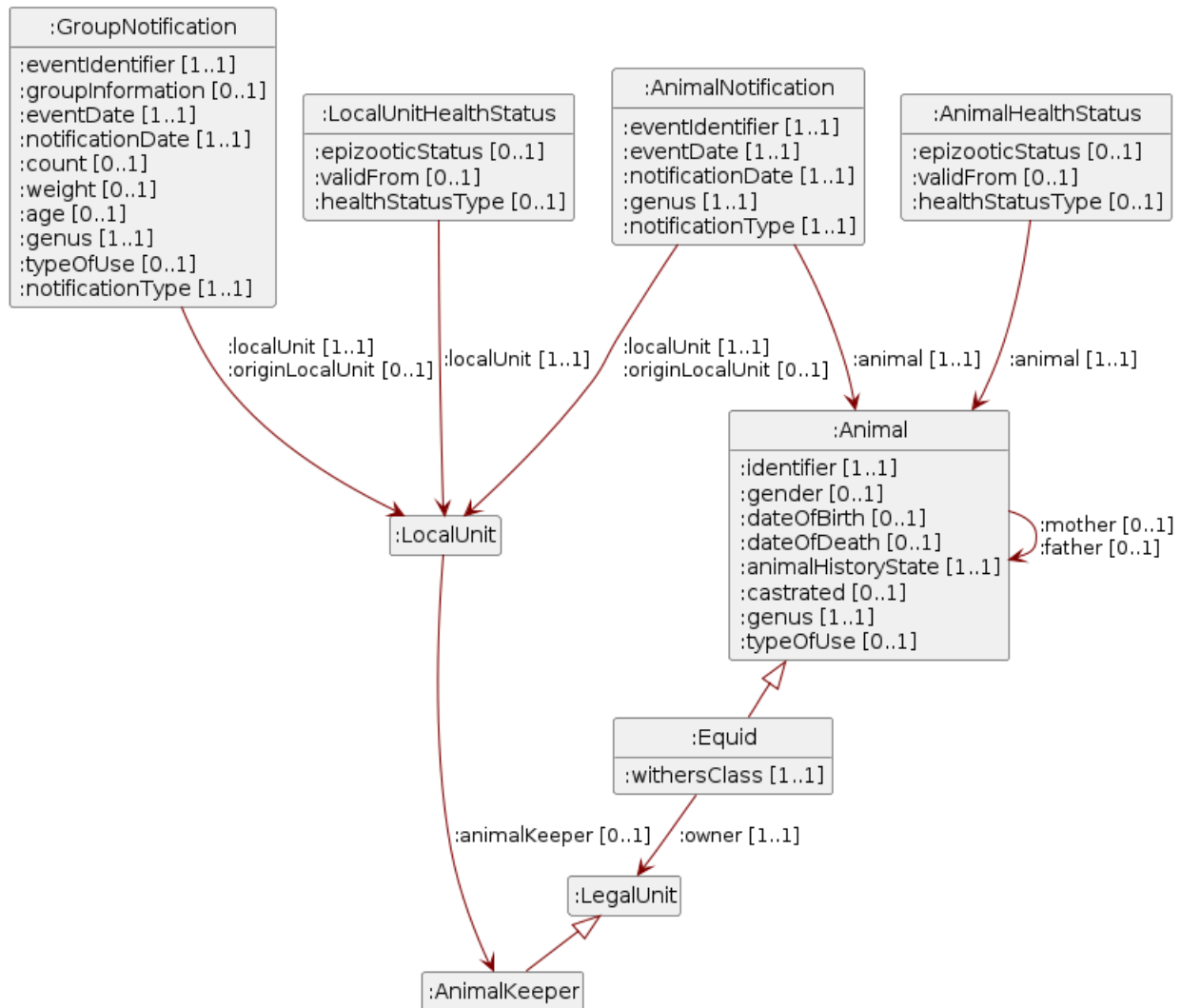
Figure 1: UML diagram of the eCH-0309 data model.
