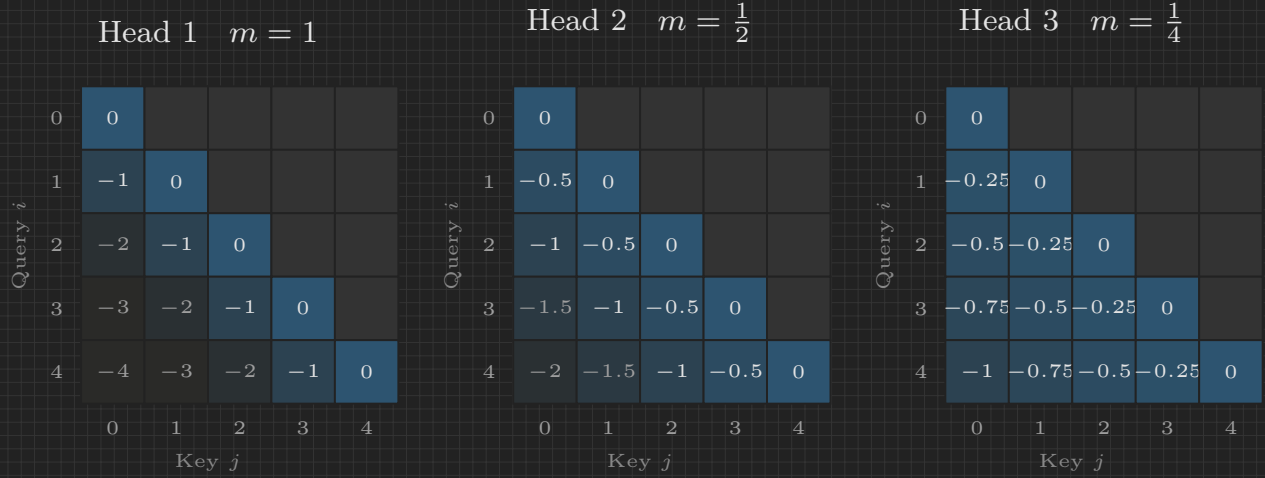
Figure 2. ALiBi just tweaks attention scores at inference with a fixed distance penalty -m(i-j) —steep slopes keep things strictly local, while smaller slopes let the model vibe with way more context.
