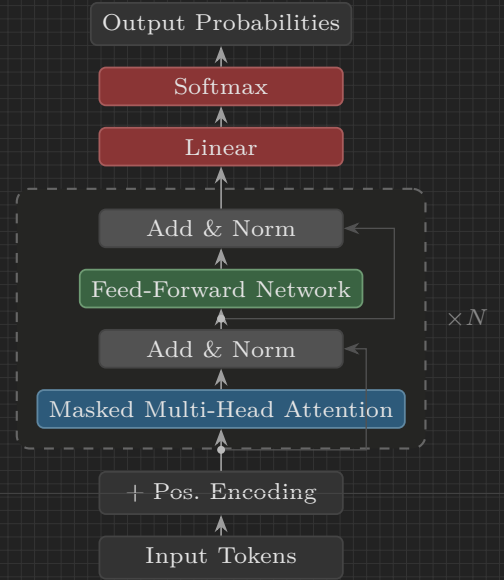
Figure 1. Decoder-only Transformer. Dashed block stacked N times.
