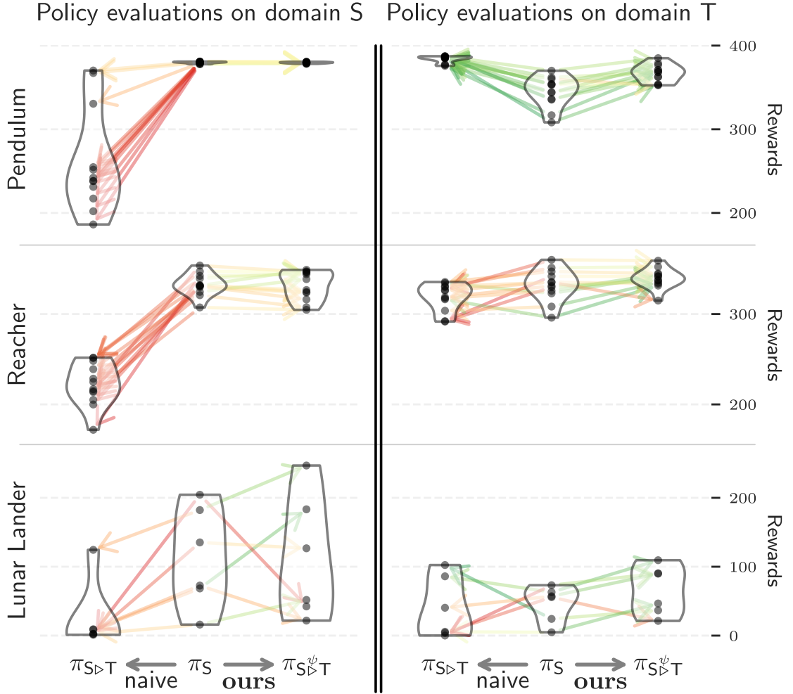
Figure 10: Comparative violin plots showing the difference of the distribution of performance of the three policies \pi_S (middle violins), the policy trained on the source domain S , \pi_{S>T} the policy trained on the source domain S and then fine tuned to the target domain T (left violins), and \pi_{S>T}^\psi the policy trained on S and then fine tuned to T using anchor critics (right violins). Arrows indicate how the agents perform after fine tuning, with red indicating a loss of performance and green showing improvement.
