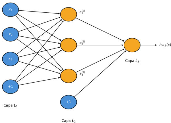
Figure 3: Xarxa neuronal multi capa.
