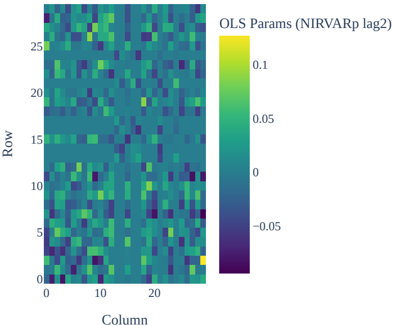
Heatmap of ols_params_NIRVARp_lag2[:, :, 0]
