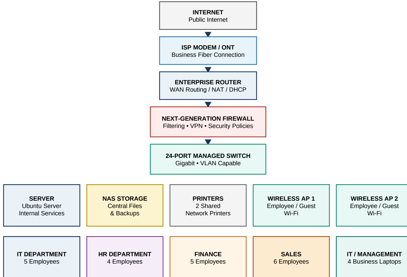
Logical VLAN Segmentation
