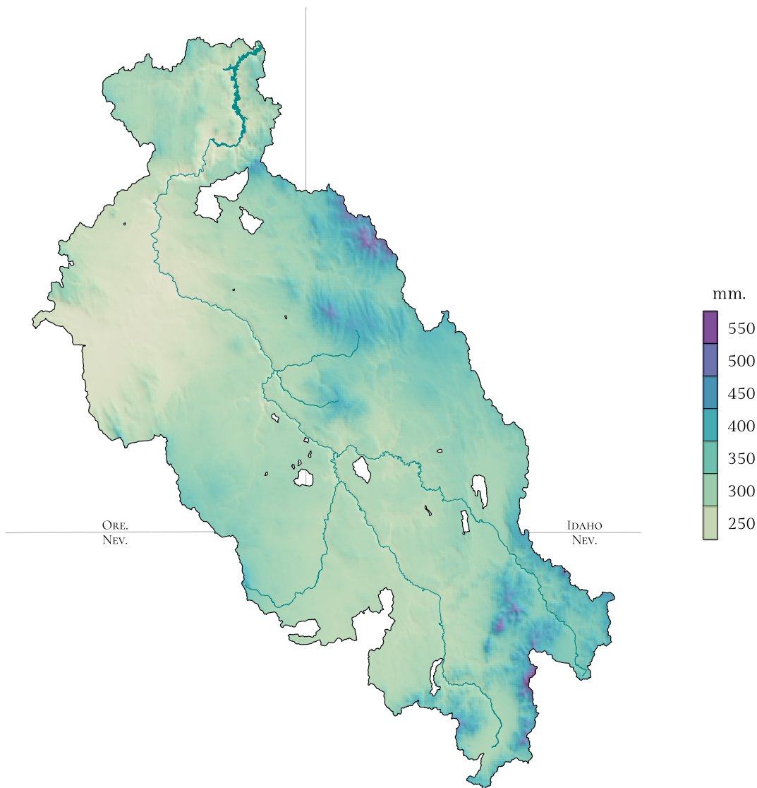
Plate 6. Average annual precipitation
