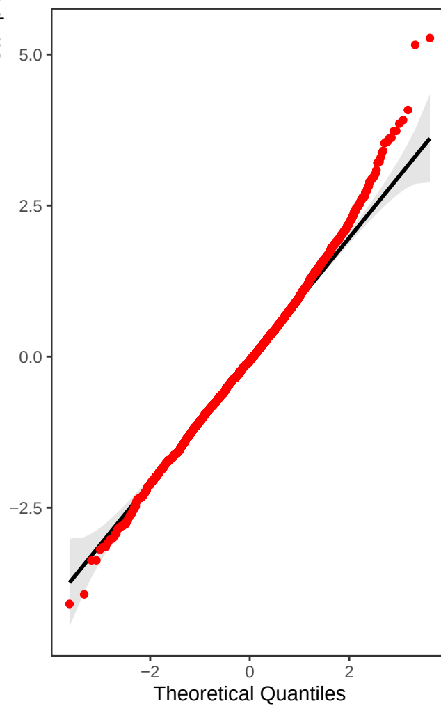
Sample Quantiles
