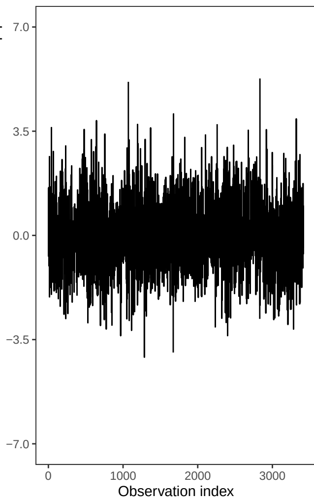
Sample Quantiles
