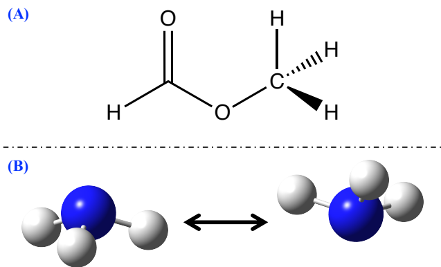
Figure A9. Examples of internal motions. (A) Structure of cis -methyl formate. As the methyl (-CH 3 ) group rotates about the C-O bond, the interaction potential between the hydrogen atoms and the oxygen atoms changes, affecting the coupling of the internal rotational angular momentum to that of the overall angular momentum of the system, perturbing energy levels and increasing spectral complexity. (B) Representation of the umbrella-like inversion motion undergone by the NH 3 molecule, which perturbs the standard rotational energy levels and adds complexity to the rotational spectra.
