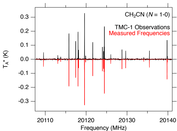
Figure A10. Observations of a single rotational transition ( N = 1-0 ) of CH 2 CN in TMC-1 from the Kaifu et al. (2004) survey in black , with the measured laboratory transitions overlaid in red . The split lines are the result of the coupling of both 1 H and 14 N hyperfine splitting of the transition.
