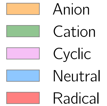
Molecule Types
