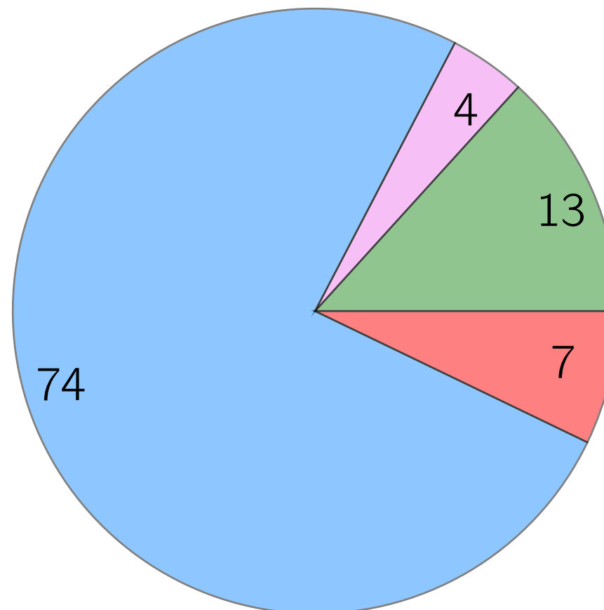
SFRs
