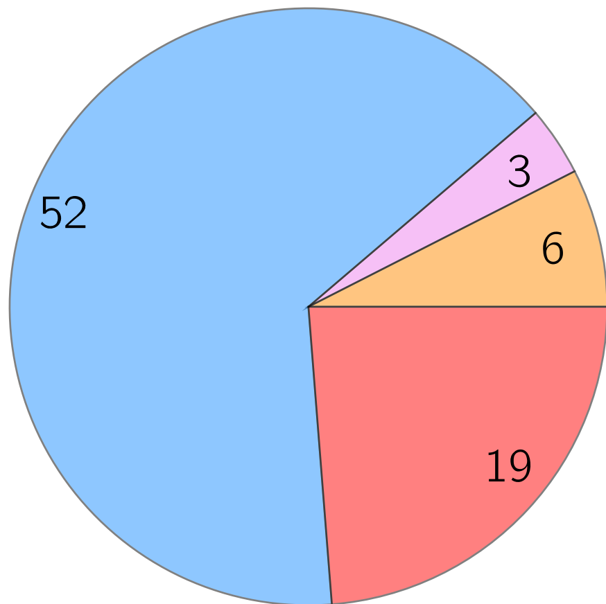
Carbon Stars
