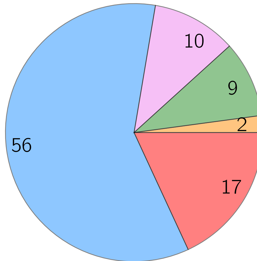
Dark Clouds
