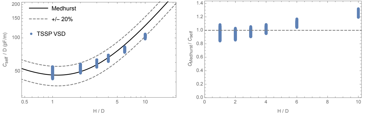
FIG. 4. Comparison of C_{\text{self}} with C_{\text{Medhurst}} of (2). (Left) Conventional log-log plot of capacitance/ D versus H/D . The VSD values of C_{\text{self}} are within roughly [-30\%, 20\%] of C_{\text{Medhurst}} . (Right) Alternative plot of the ratio of values versus H/D , for direct comparison with later plots.
