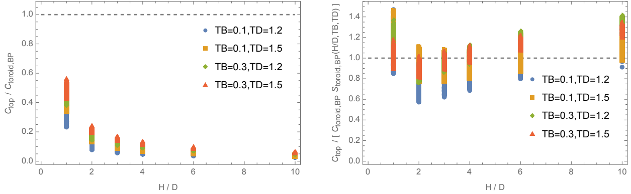
FIG. 10. Comparison of estimates for C_{\text{load}} using the TSSP VSD and a common formula. (Left) Ratio of the extracted C_{\text{top}} of (25) over the estimate C_{\text{toroid,BP}} of (C10). (Right) Adjusting the ratio using the fitted correction factor S_{\text{toroid,BP}} of (C12) removes most of the dependence on H/D .
