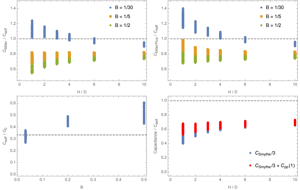
FIG. 5. Tests of the Miller self-capacitance (12). (Top left) C_{\text{Miller}} versus H/D for different solenoid heights B above the ground plane. (Top right) Adding a gradient correction (23): C_{\text{MillerPlus}} = C_{\text{Miller}} + C_{\text{pp}}(1) . (Bottom left) Alternate plot of C_{\text{self}}/C_0 versus B to compare with the ideal Miller value of 1/3 . (Bottom right) Comparison using a theoretical estimate (14) for C_0 .
