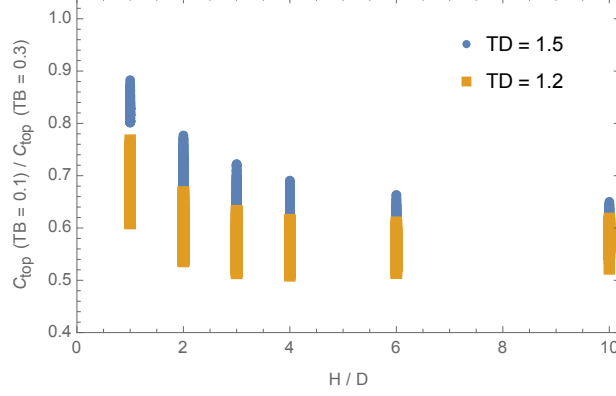
FIG. 2. Ratio of the extracted capacitance C_{\text{top}} of (25) for identical toroid electrodes at two different heights TB above the solenoid. Raising the height generally decreases C_{\text{top}} by up to almost half, depending on H/D and the toroid diameter TD. The overlap of thousands of data points covering all parametric variations gives the appearance of lines at each discrete value of H/D used in the VSD. Data points for different TD overlap significantly at large H/D .
