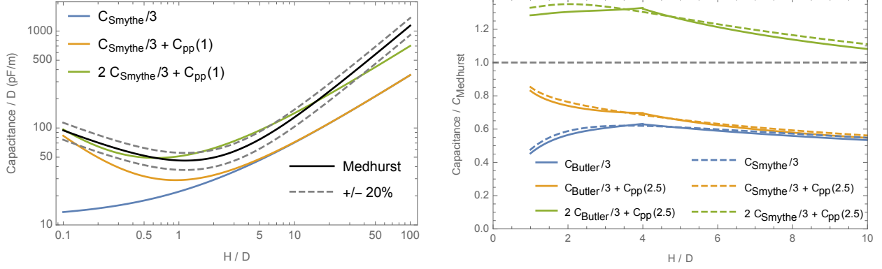
FIG. 7. Comparison of the Miller self-capacitance (12) and C_{\text{Medhurst}} using the theoretical values (13) or (14) for C_0 . (Left) Conventional log-log comparison using (14). The results are similar for (13). (Right) Alternative linear plot of ratio.
