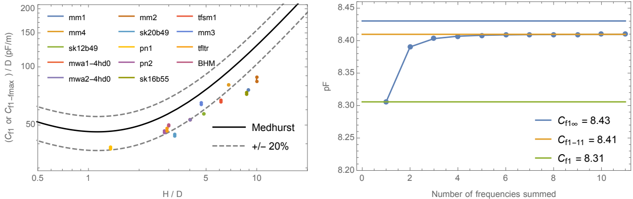
FIG. 8. Tests of the frequency-based model (15) and its variations using experimental values. (Left) Using measurements provided in the TSSP's online documentation 5 and from Ref. 19 ("BHM"). For each solenoid, there are points for both (18) and a partial sum of (15) up to the highest reported resonance. (Right) Sum convergence using measured frequencies from Ref. 19.
