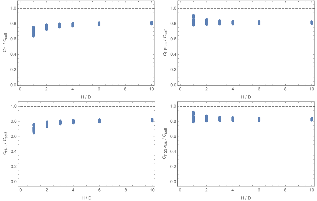
FIG. 6. Tests of the frequency-based model (15) and its variations. (Top left) Using the first resonant frequency with (18). (Top right) Adding the gradient correction C_{\text{pp}}(1) of (23). (Bottom left) Using the first resonant frequency with (20), which has a slight correction. (Bottom right) Using the first three resonant frequencies with (19), and adding the gradient correction C_{\text{pp}}(1) .
