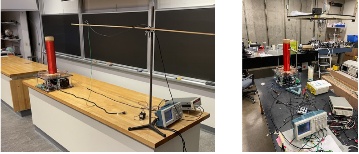
FIG. 11. Pictures of the two measurement setups used for Appendix C3. Both setups used the same Tesla coil. (Left) “Setup A” in a classroom. (Right) “Setup B” in a laboratory with a metal stand nearby holding a probe. Both pictures show a configuration with the toplayer removed.
