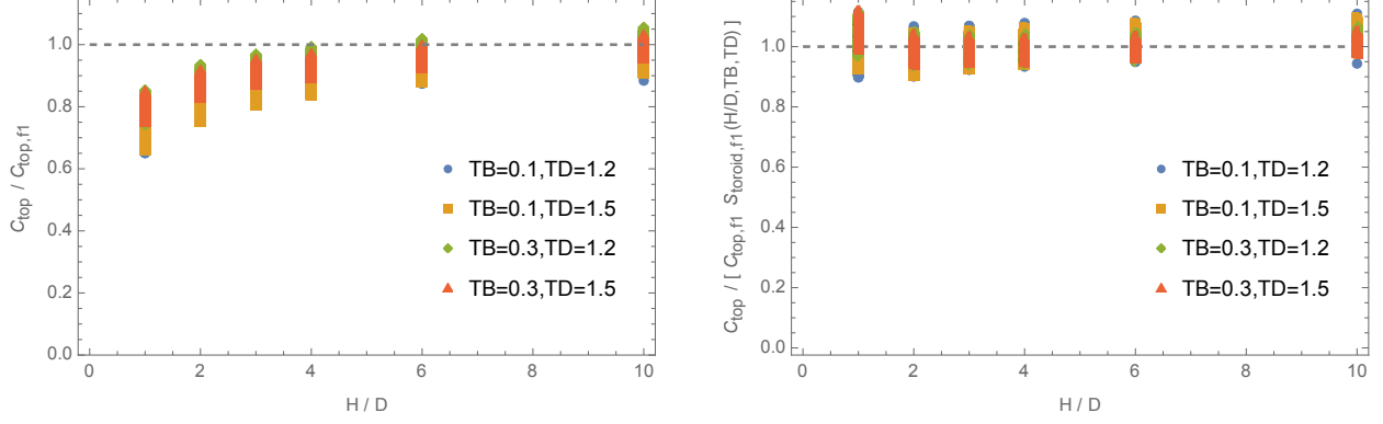
FIG. 9. Comparison of estimates for C_{\text{load}} using electrostatic capacitances or resonant frequencies. (Left) Ratio of the electrostatic estimate C_{\text{top}} of (25) over the resonant-frequency estimate C_{\text{top},f1} of (C1) versus H/D . (Right) Adjusting the ratio using the fitted correction factor S_{\text{toroid},f1} of (C3) removes most of the dependence on H/D .
