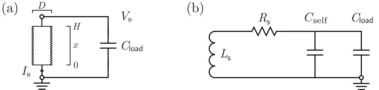
FIG. 1. Solenoid self-capacitance. (a) Physical setup of a grounded solenoid inductor with a lumped capacitive load C_{\text{load}} . (b) Equivalent circuit intended only to determine the lowest resonant frequency \omega_1 = 2\pi f_1 , which includes a “self-capacitance” C_{\text{self}} for the solenoid in addition to resistance R_s and self-inductance L_s .
