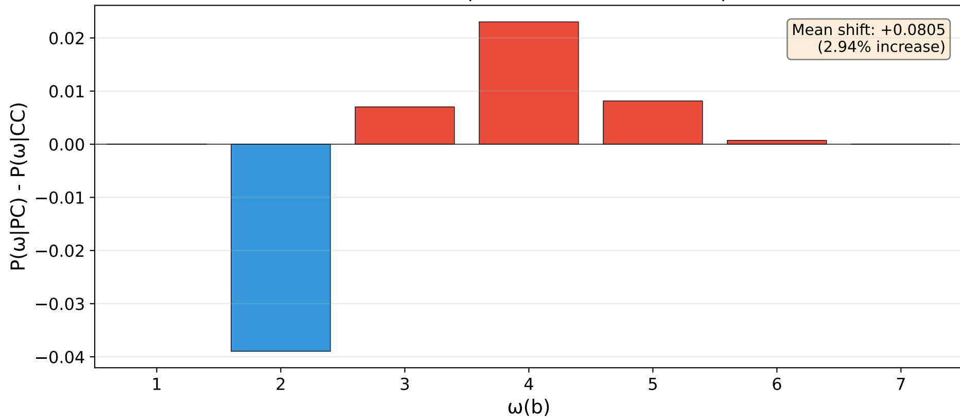
Distribution shift: PC composites have more prime factors (red = PC more frequent, blue = CC more frequent)
