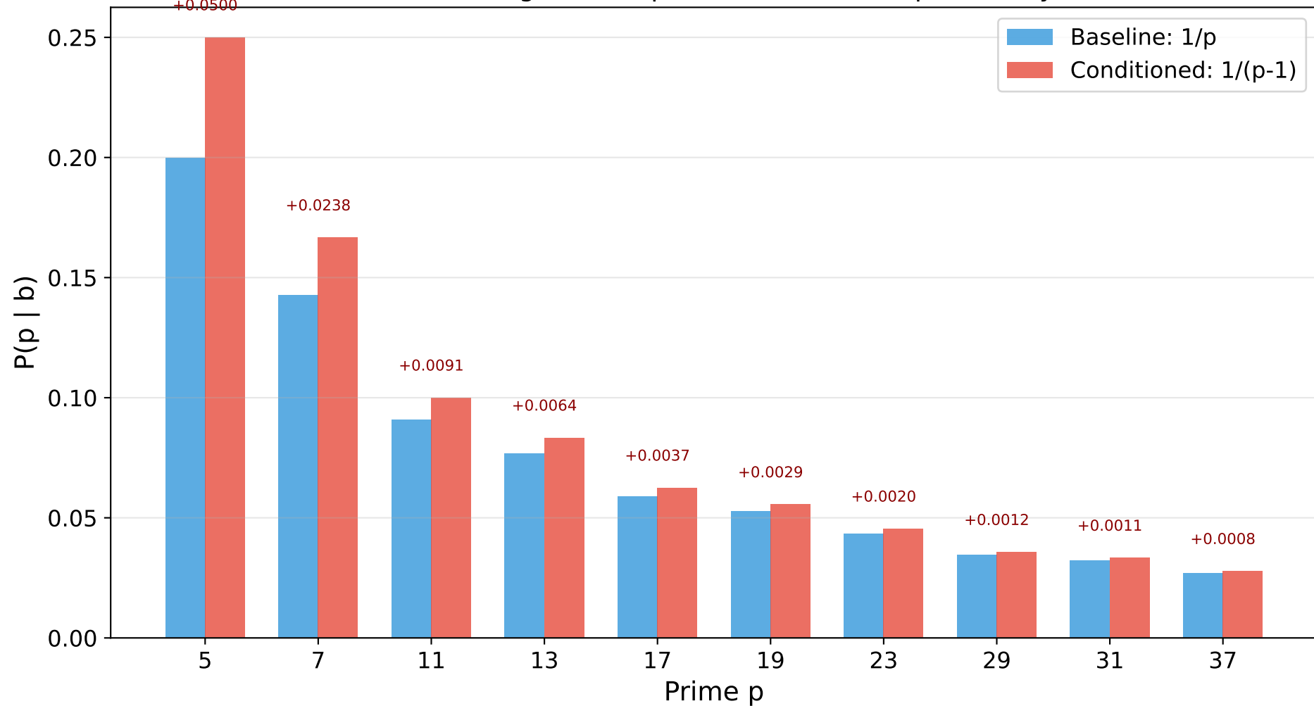
Per-prime divisibility probability (conditioning on "a is prime" boosts each probability)
