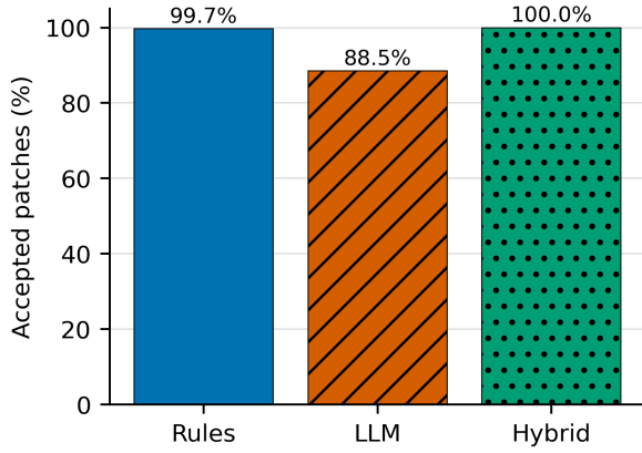
Figure 4. Verifier acceptance across deterministic, LLM-backed, and hybrid proposer modes; the rules-only 5k evidence in this comparison is an archived verifier-record snapshot rather than a current verifier rerun.
